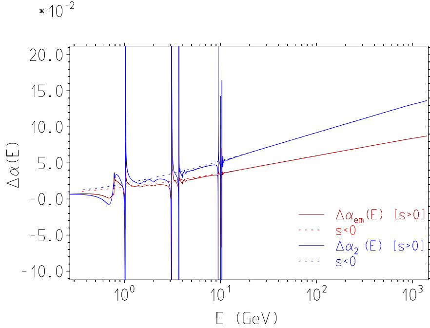
Fig. 1. -\Delta\alpha_{\text{em}}(E) and \Delta\alpha_2(E) as functions of energy E in the time-like and space-like domain. The smooth space-like correction (dashed line) agrees rather well with the non-resonant “background” above the \phi -resonance (kind of duality). In resonance regions as expected “agreement” is observed in the mean, with huge local deviations.
