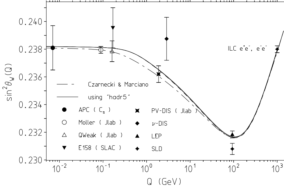
Fig. 2. – \sin^2 \Theta_W(Q) as a function of Q in the space-like region. Hadronic uncertainties are included but barely visible. Uncertainties from the input parameter \sin^2 \theta_W(0) = 0.23822(100) or \sin^2 \theta_W(M_Z^2) = 0.23156(21) are not shown. Future ILC measurements at 1 TeV would be sensitive to Z' , H^{\pm\pm} etc.
